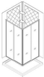
Framed Rectangular Shower Enclosure
